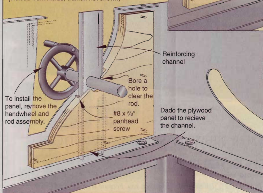
Newer Craftsman and Ridgid saws (viewed from inside, trunion not shown)
